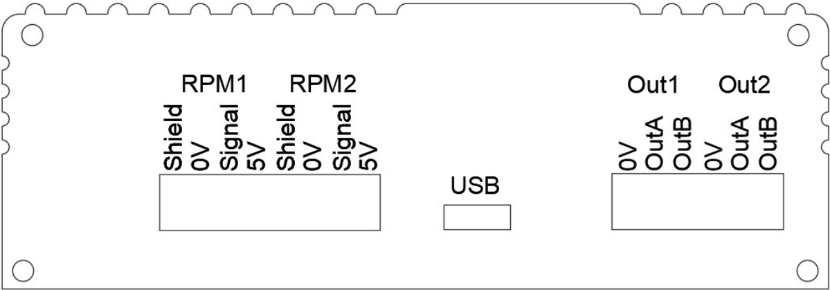
Figure 1 Standard v4 connections
