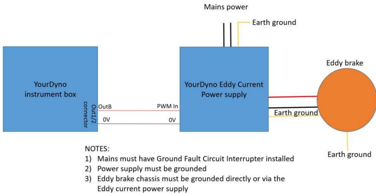
Figure 5 Use OutB for Standard v4 and Out for Standard v5
