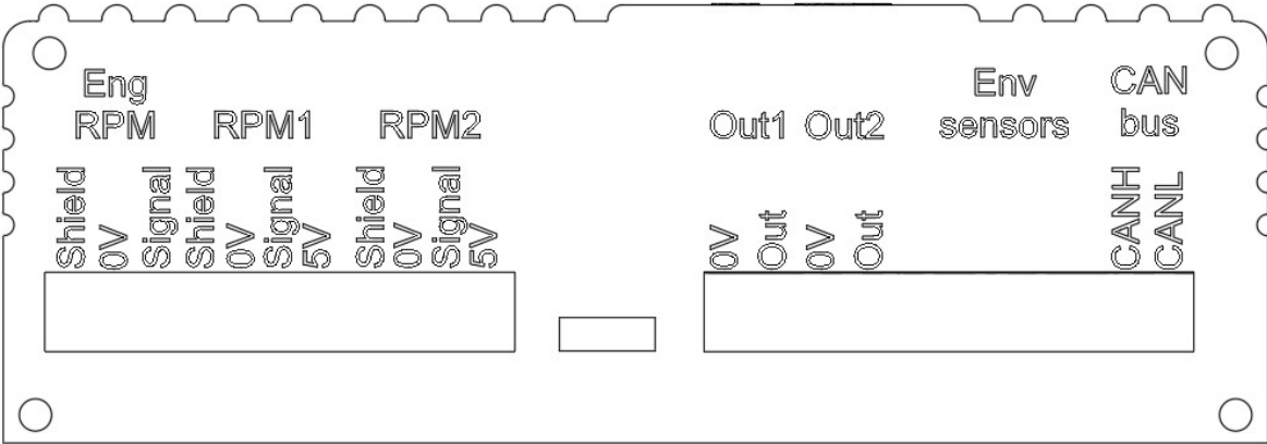
Figure 2 Standard v5 connections
