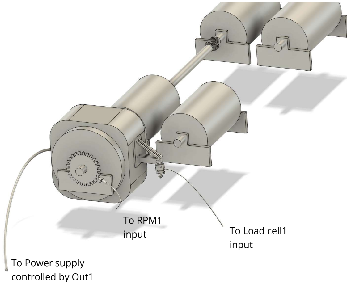
Example of single axis roller based eddy braked dyno
